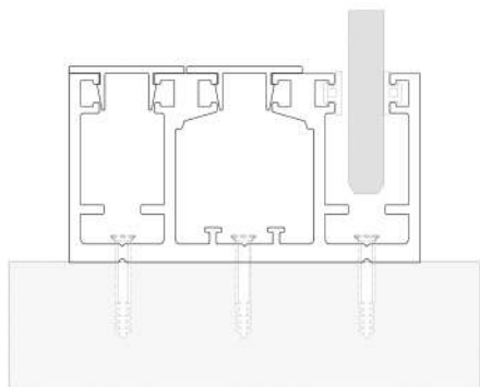
G107 Profile
