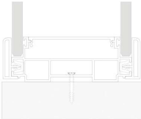
G201 Profile
