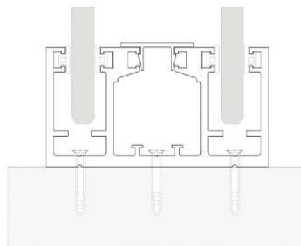
G203 Profile
