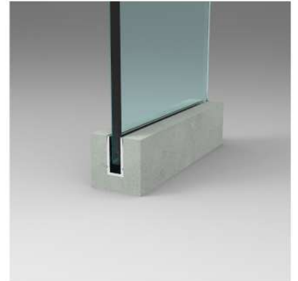
G102 Profile
