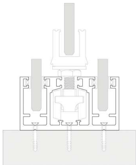
G204 Profile
