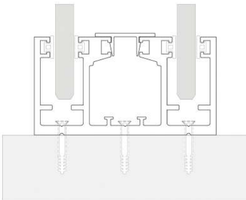
G203 Profile
