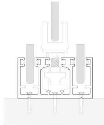
G204 Profile
